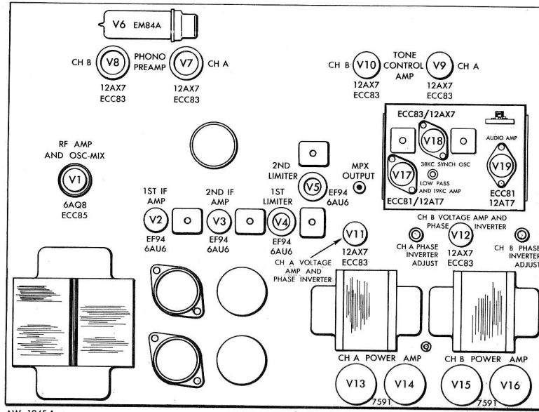
FIGURE 2. Tube layout.
